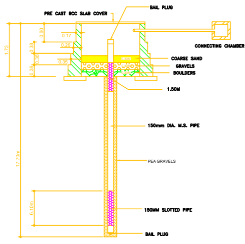
DETAIL OF RAIN WATER HARVESTING (RWH) (NOT TO SCALE)
