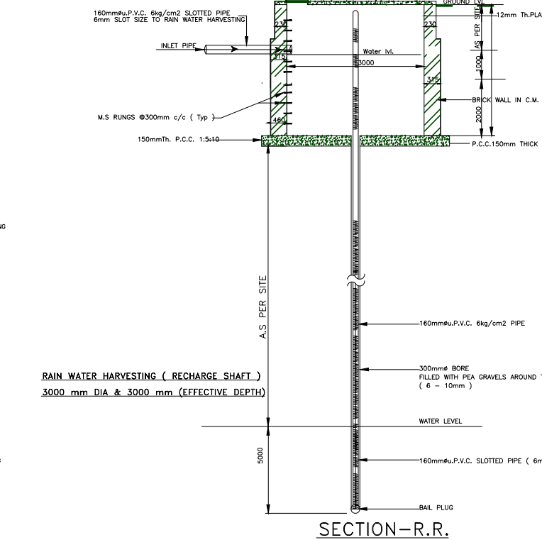
SECTION-R.R.
