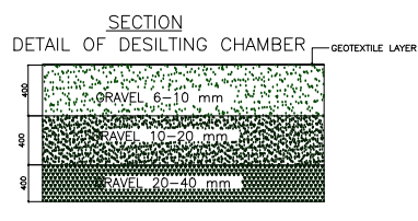
DETAILS OF FILTER BED
