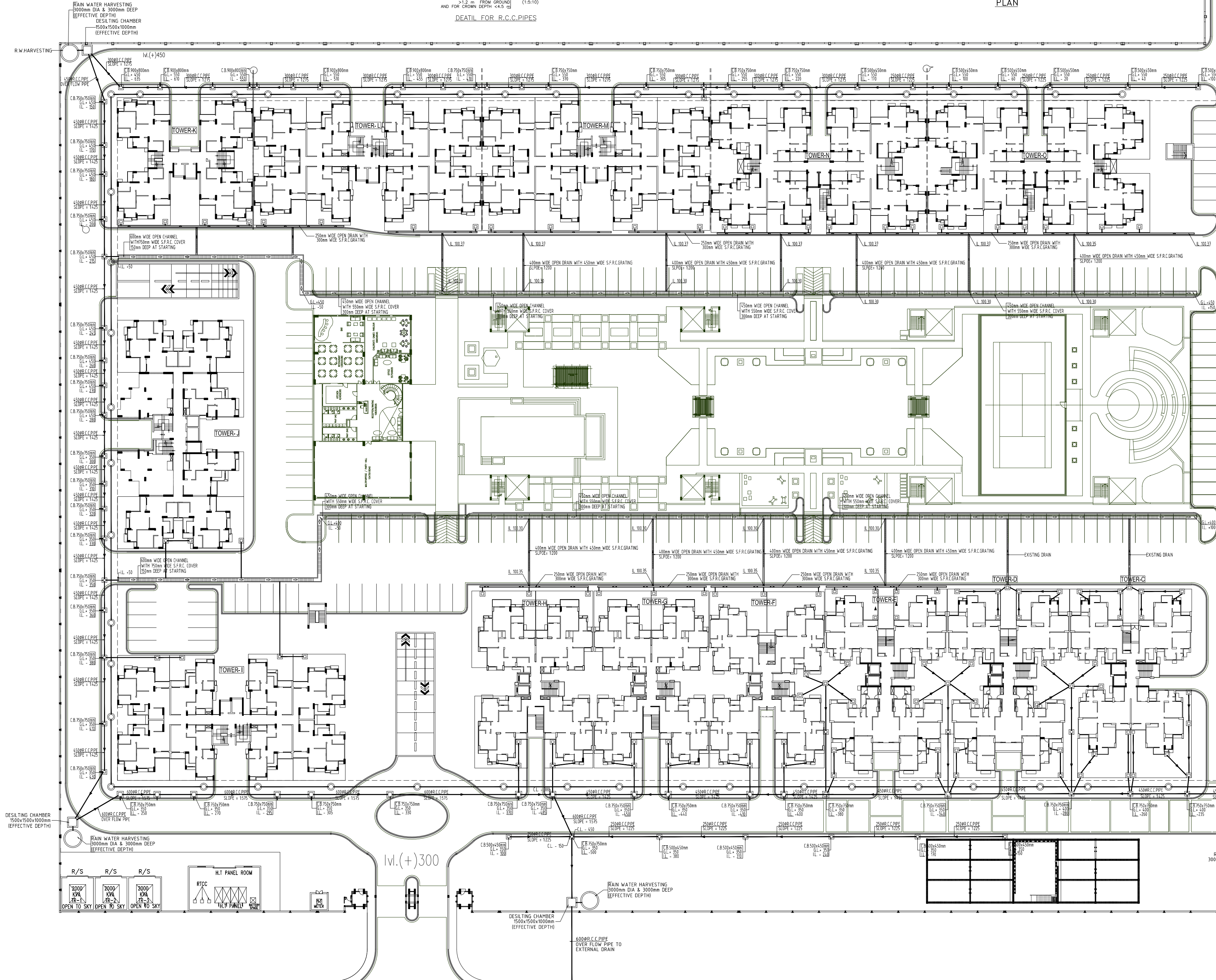
PLAN
