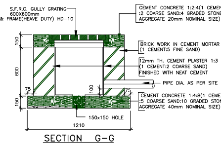
SECTION G-G
