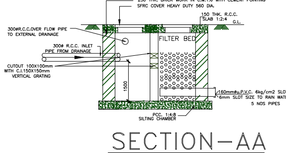
DESILT CHAMBER DETAILS
