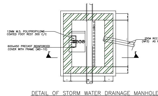
DETAIL OF STORM WATER DRAINAGE MANHOLE
