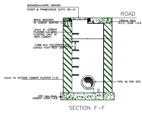
SECTION F-F
