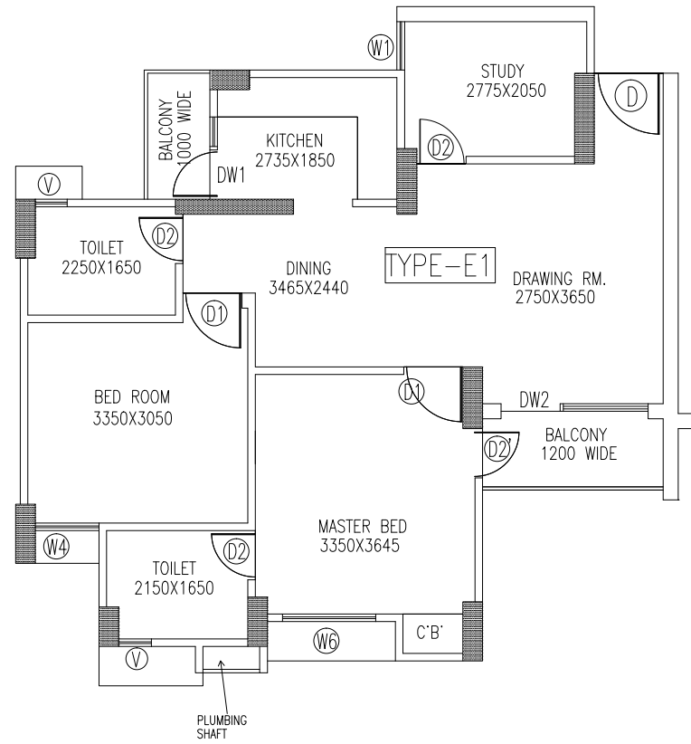
TYPE-E1 2 BED + STUDY UNIT
