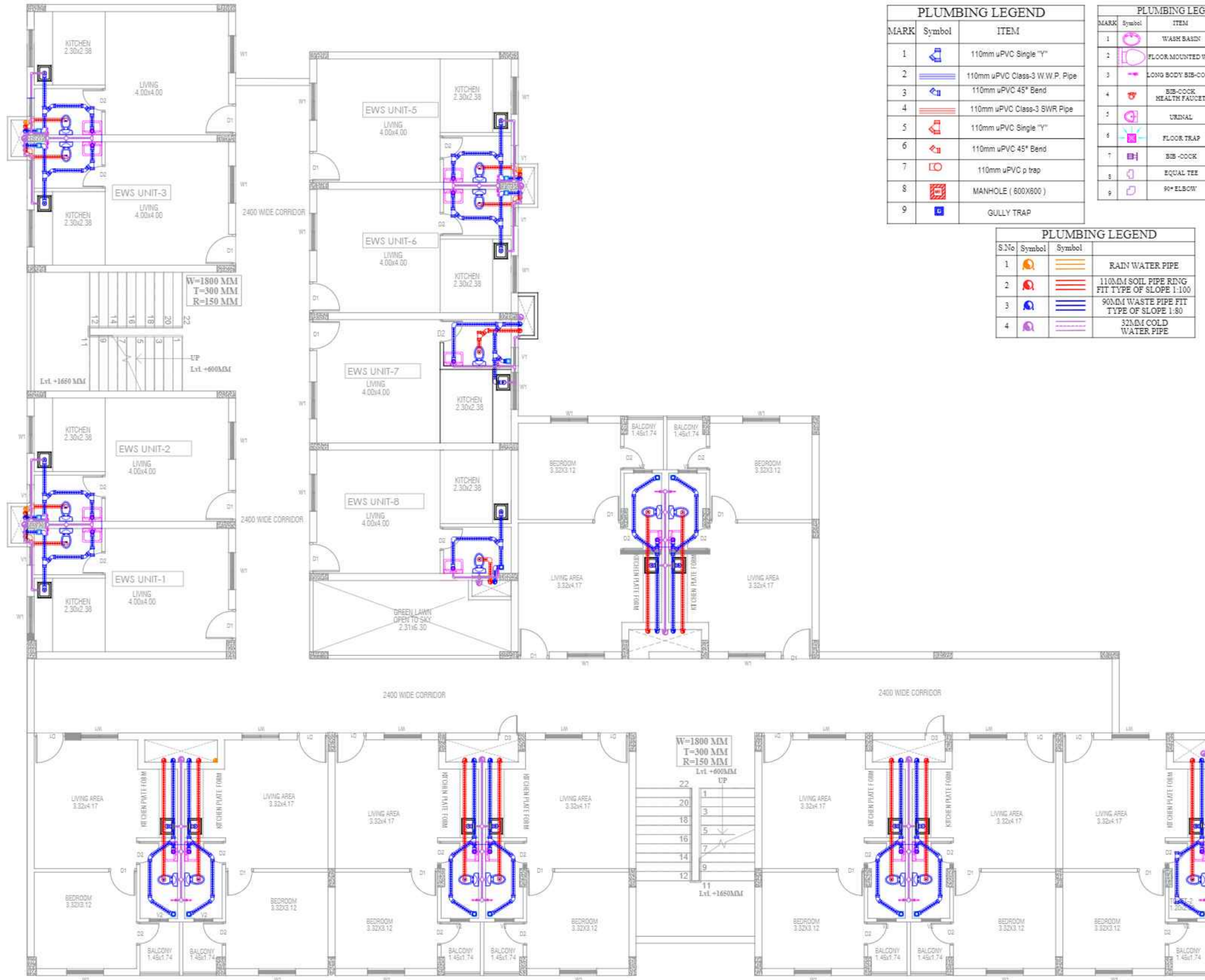
THIRD FLOOR PLAN L.I.G. AND E.W.S
