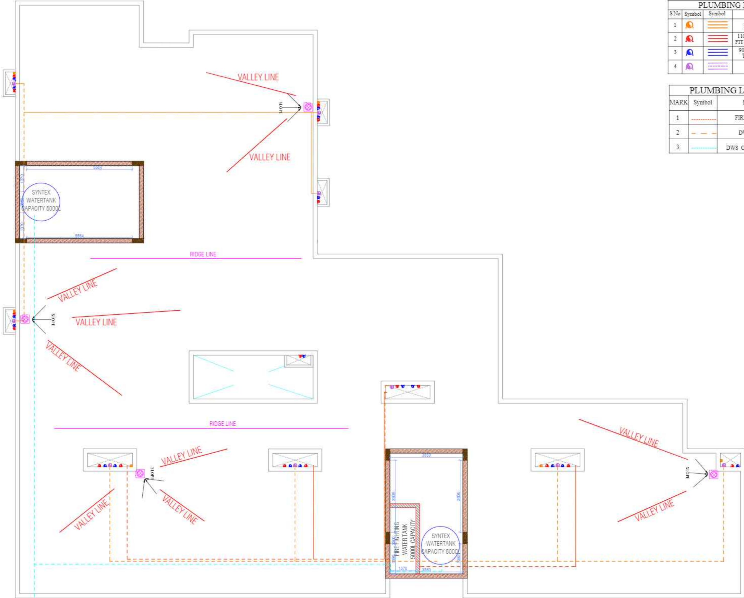
TERRACE FLOOR PLAN L.I.G. AND E.W.S
