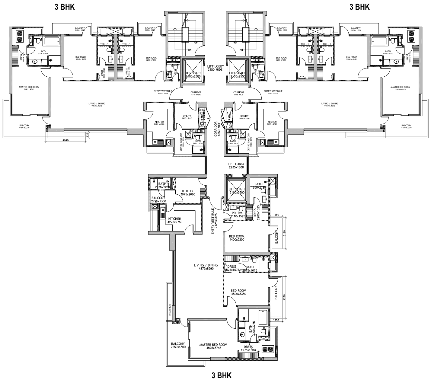
Tower 2 TYPICAL FLOOR PLAN
