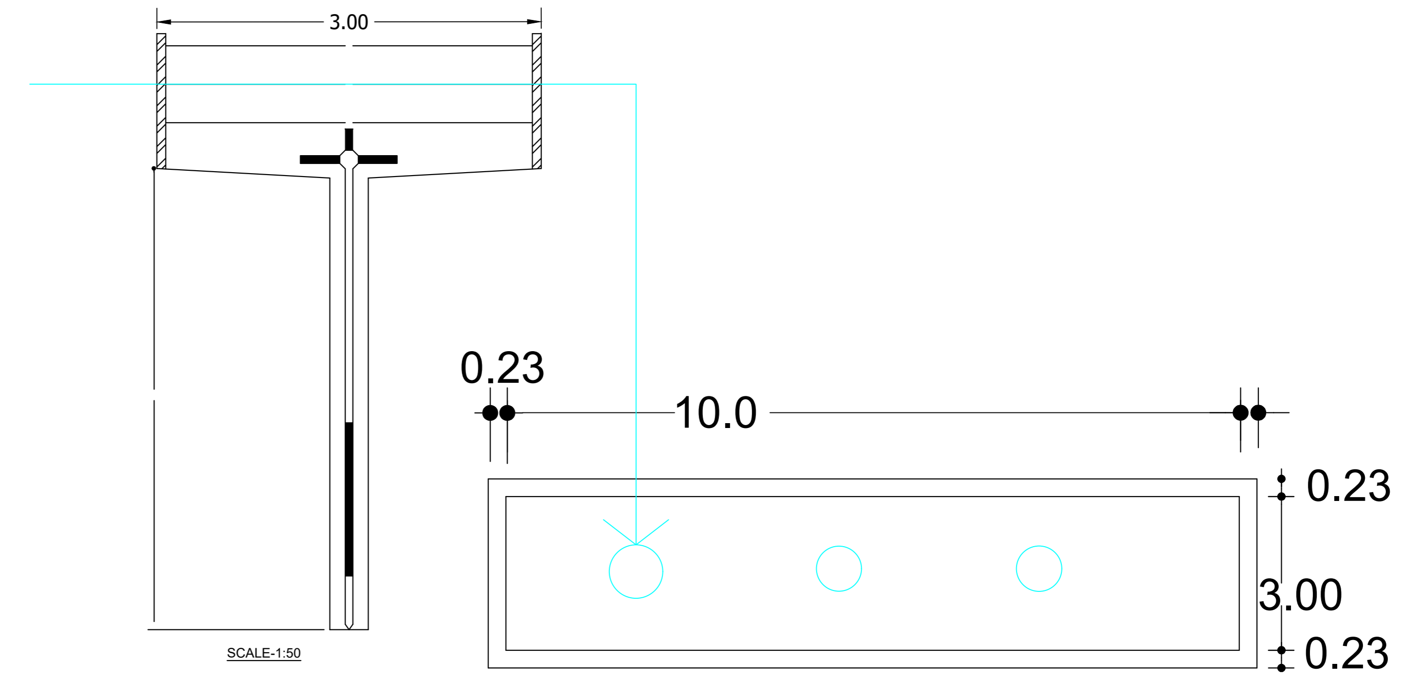
SEC.R.C. SHAFT PLAN LATERAL RECHARGE TANK DETAIL OF RAIN WATER HARVESTING SYSTEM
