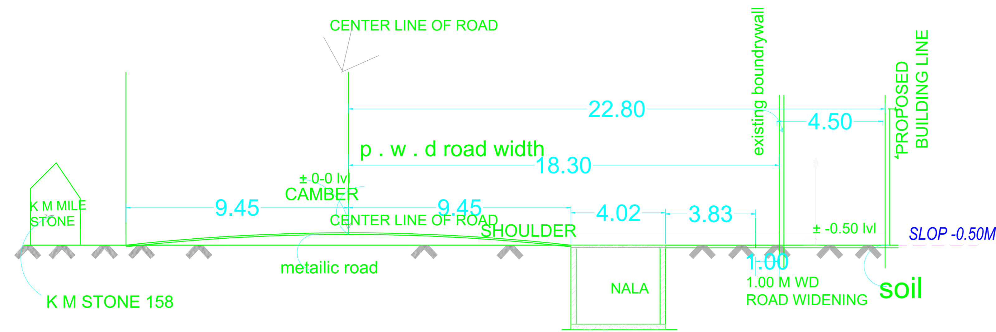
X-SECTION OF OLD N . H-24 ( CITY PORTION ) (SCALE 1:200)
