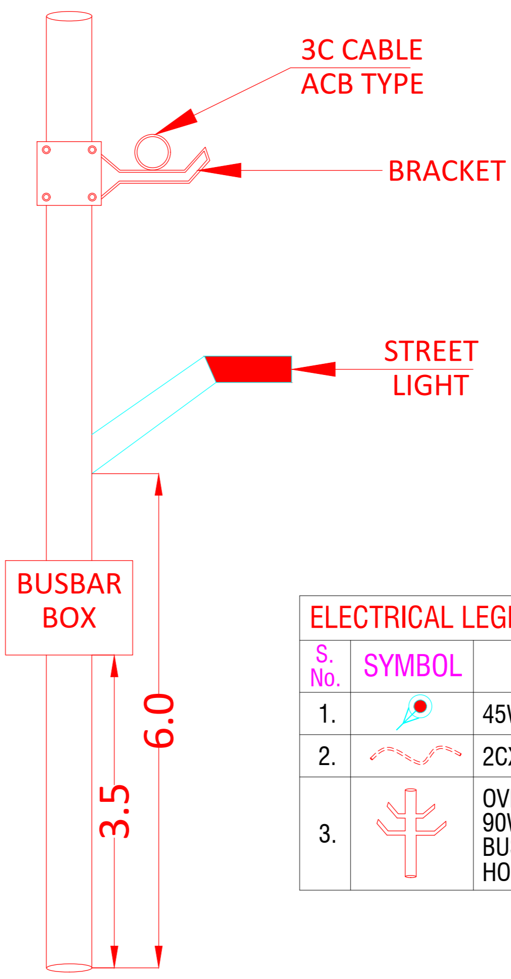
OVERHEAD LT CABLE POLE SECTION
