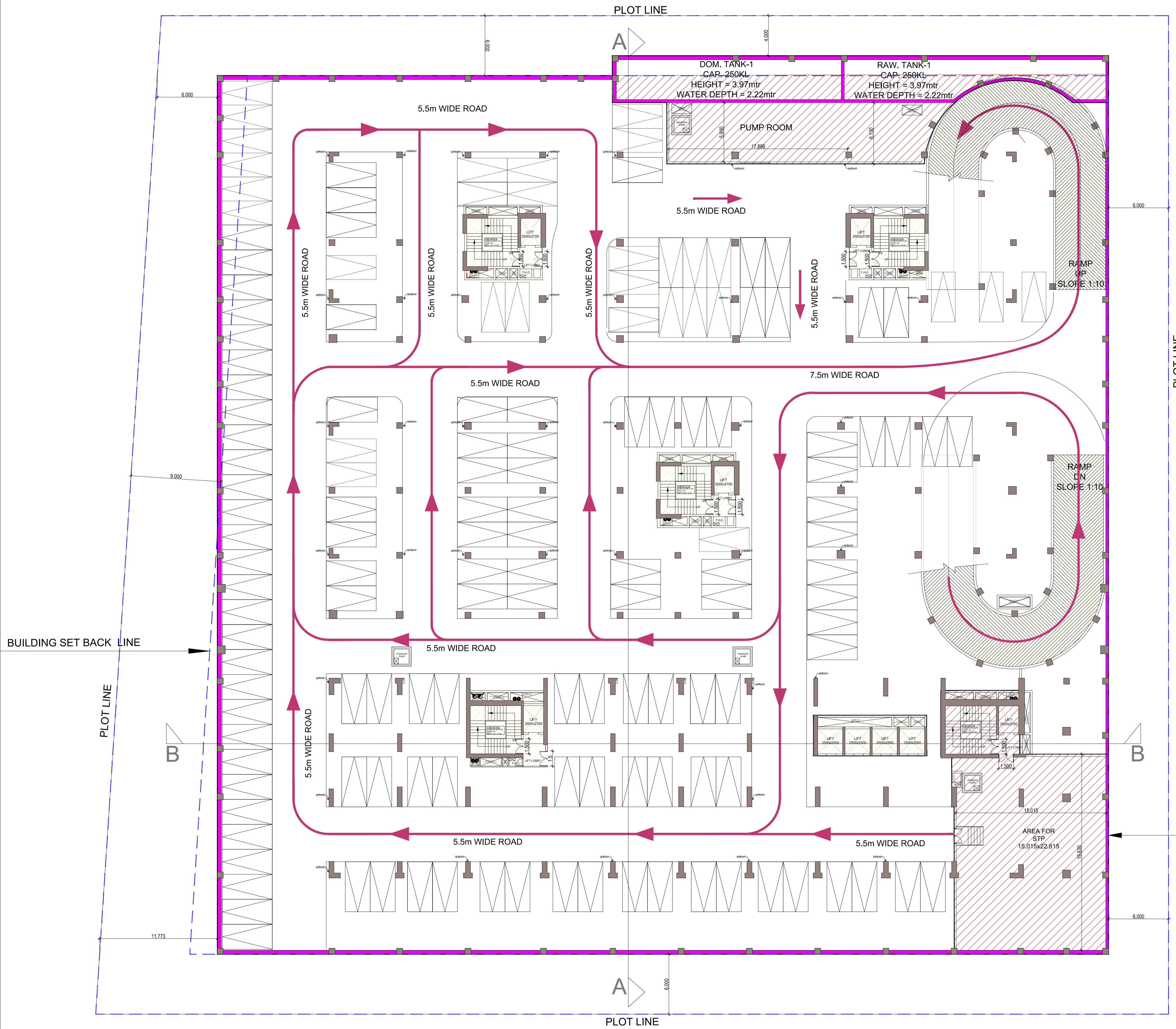
2ND. BASEMENT PLAN
