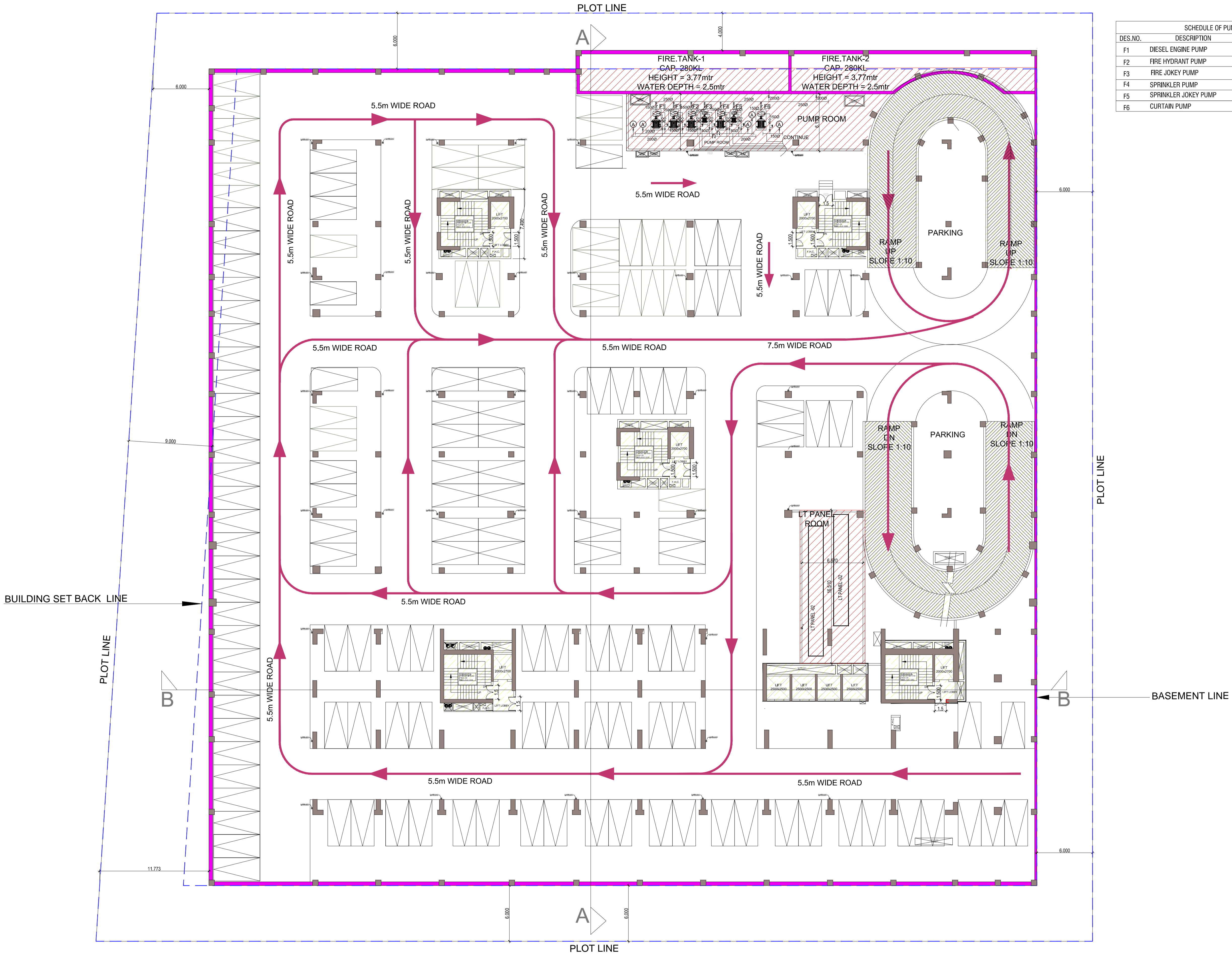
1ST. BASEMENT PLAN
