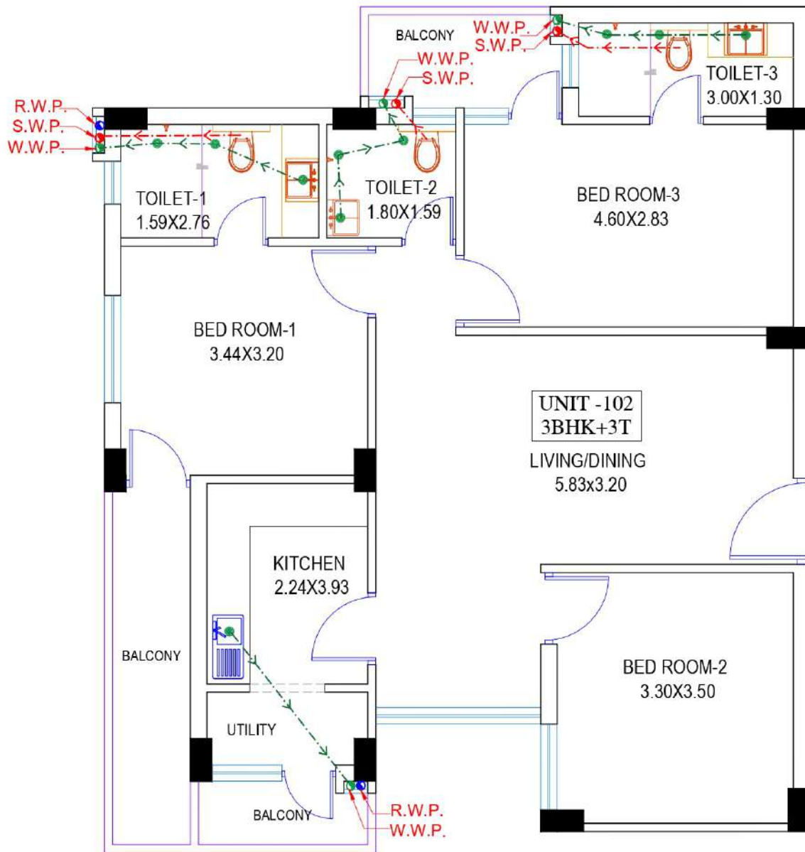
TOWER 1B (UNIT -102, 3BHK+3T)
