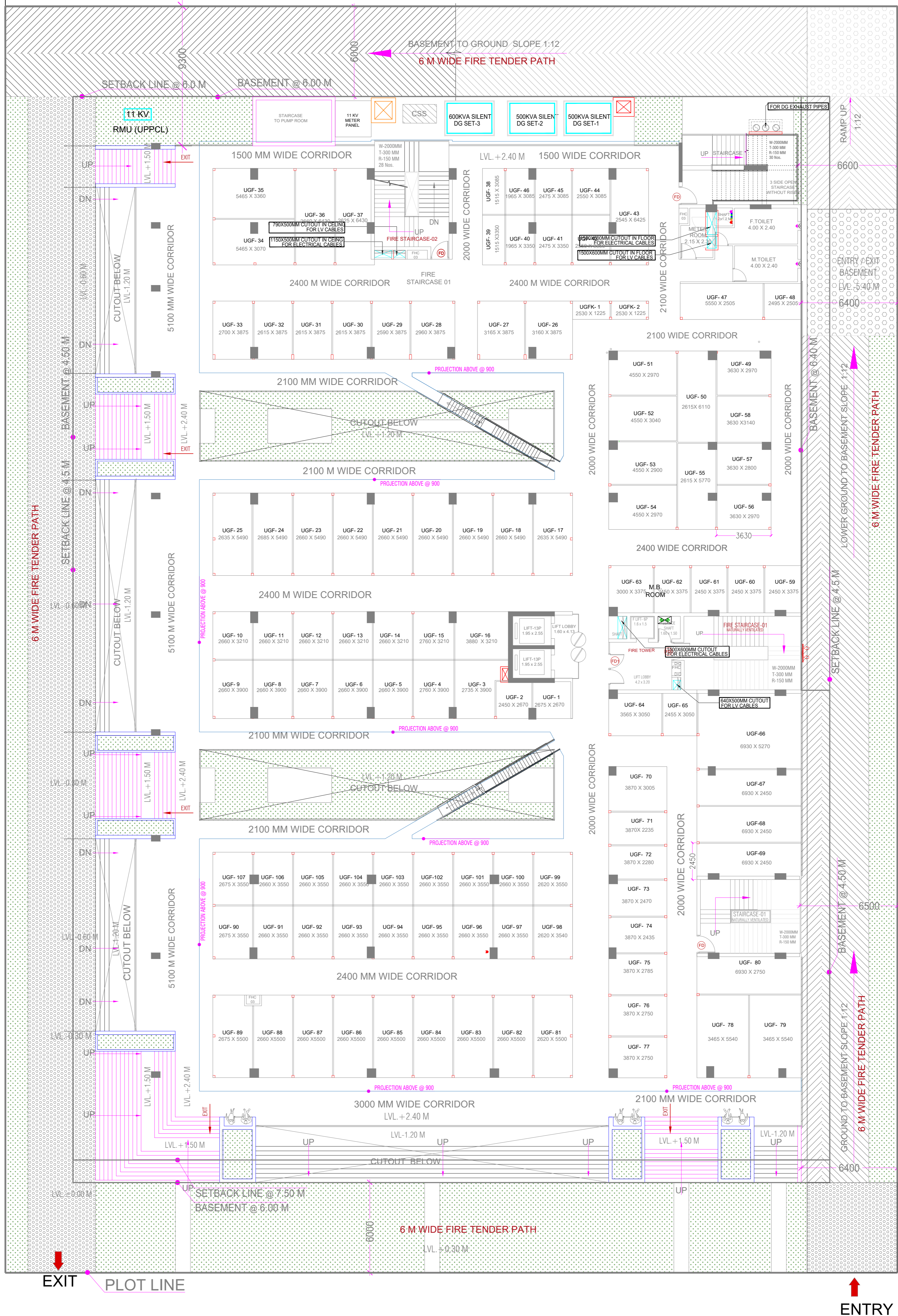
UPPER GROUND FLOOR PLAN
