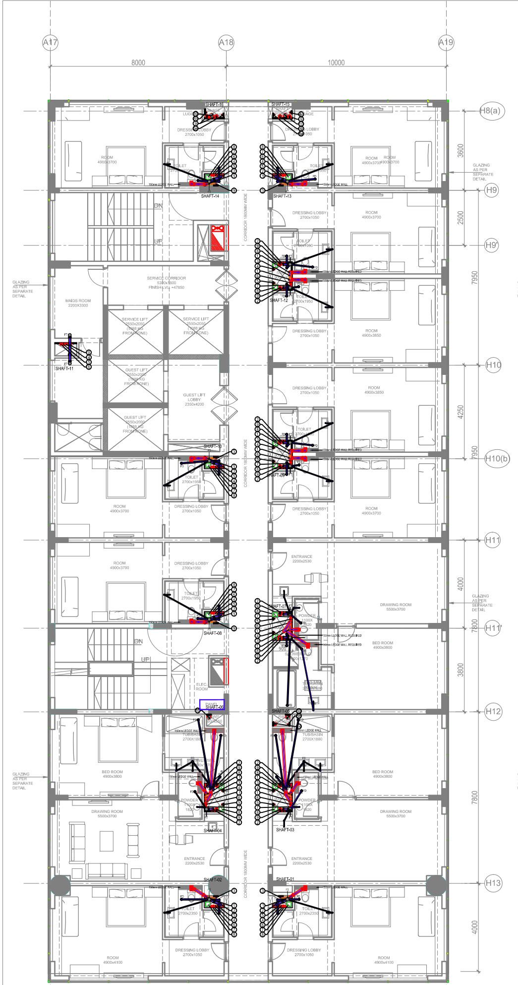
11TH FLOOR ARCHITECTURAL
