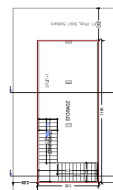
BASEMENT FLOOR PLAN (Proposed) (SCALE 1:100)
