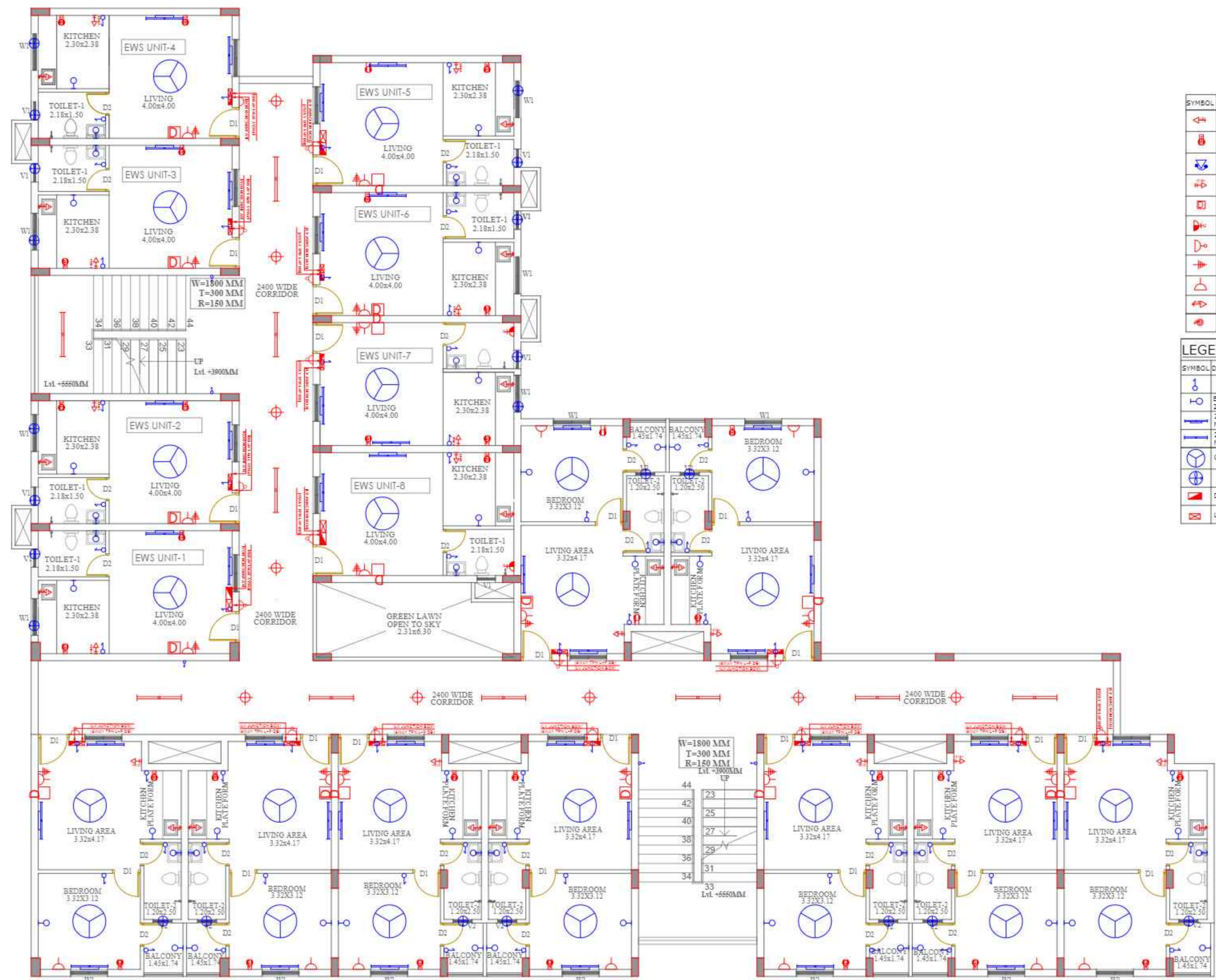
SECOND FLOOR PLAN L.I.G. AND E.W.'S SECTION
