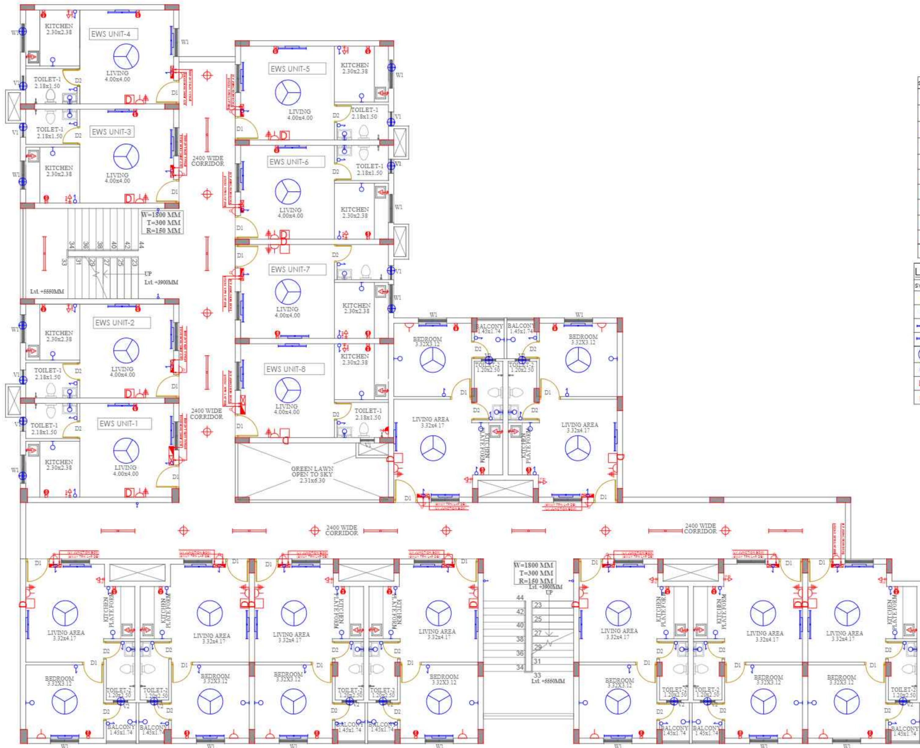
THIRD FLOOR PLAN L.I.G. AND E.W.S. SECTION
