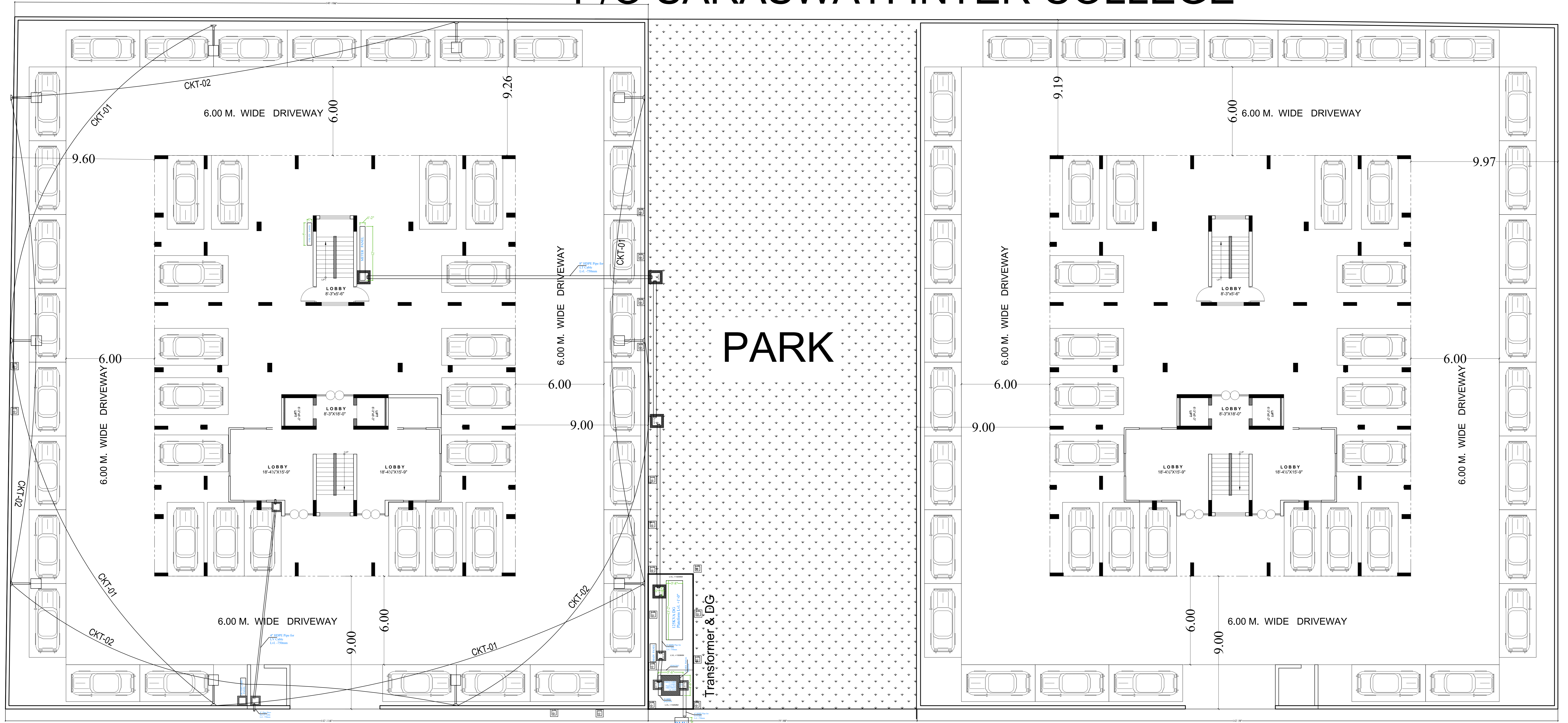
PROPOSED GROUP HOUSING 01 STILT FLOOR PLAN
