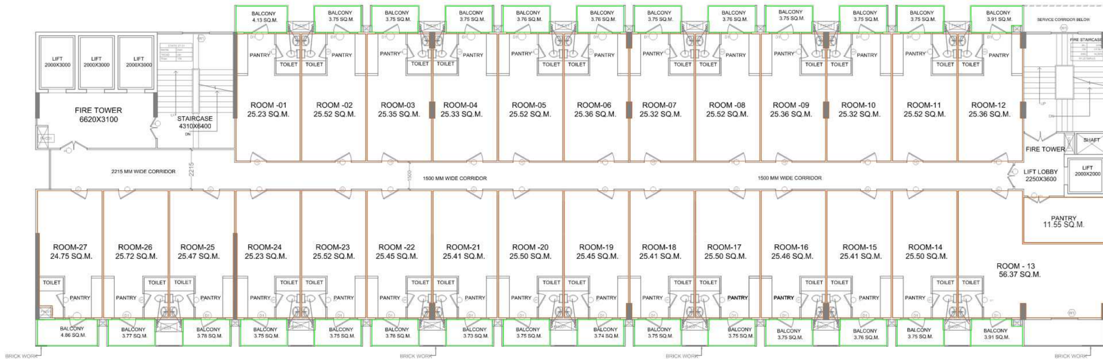
10th to 11th FLOOR PLANS LVL + 36000 to LVL + 39000
