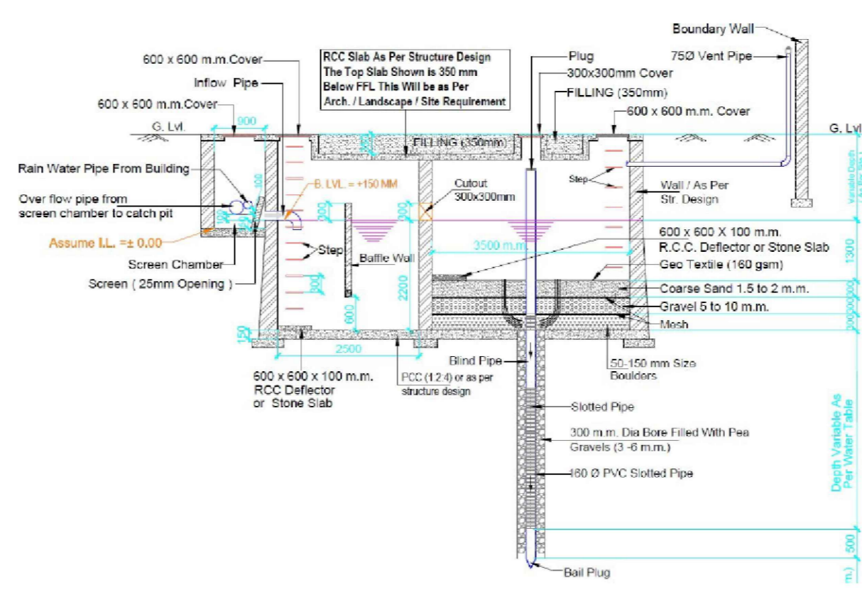
Figure No. 4: Rain Water Harvesting Pit Design
