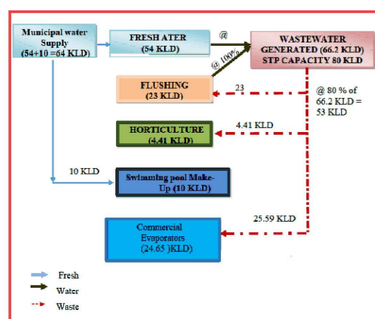
Figure No. 1: Water Balance Diagram for Non-Monsoon Seasons
