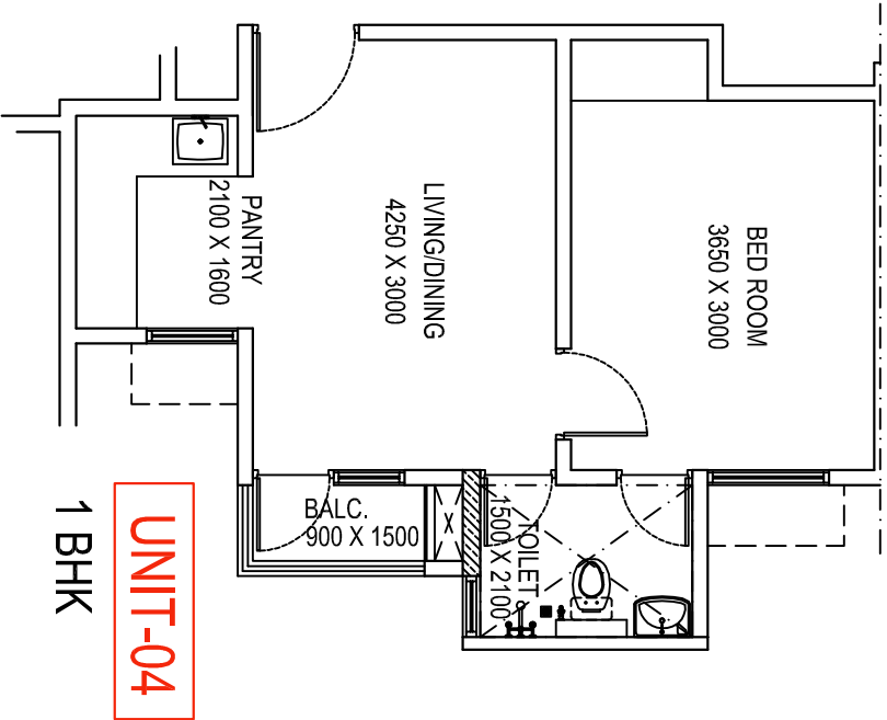
TYPICAL FLOOR (1ST. TO 14TH.) UNIT PLAN
