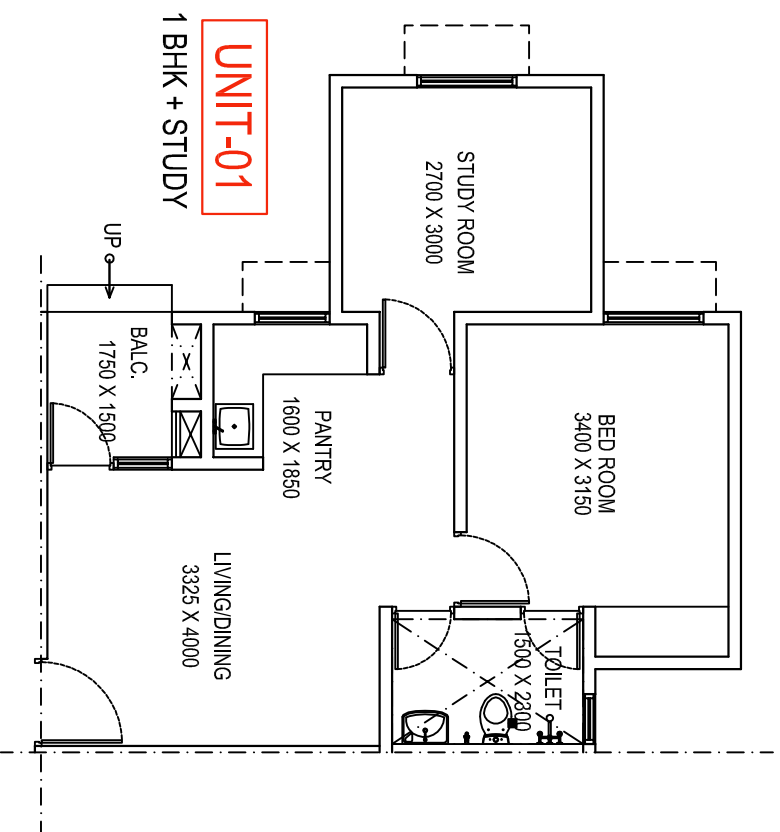
GROUND FLOOR UNIT PLAN
