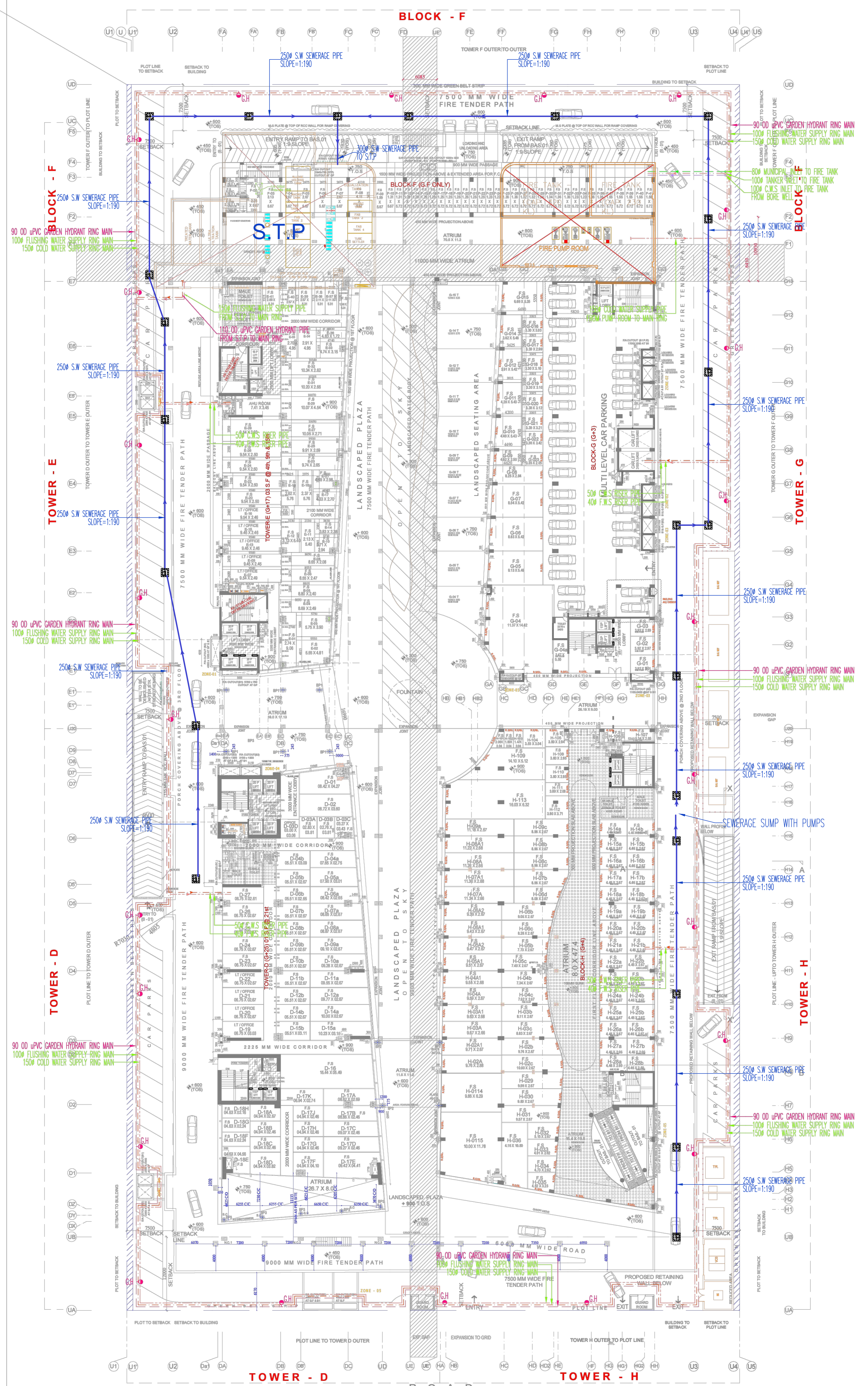
GROUND FLOOR PLAN @ +900
